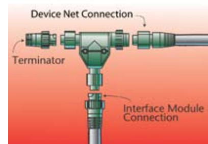
Connect to NMEA 2000 Cable. Kit includes Device Net Connectors..
