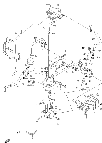
DF15A20A P01 013_009 FUEL PUMP
