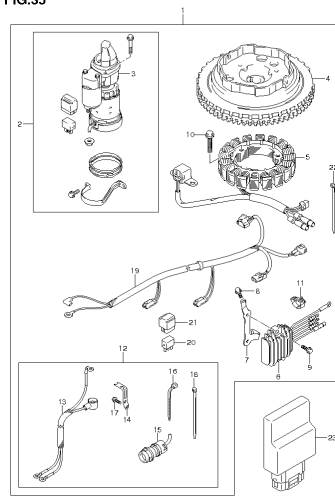
DF15A 2/A P01 013_035 OPT STARTING MOTOR (MANUAL STARTER)
