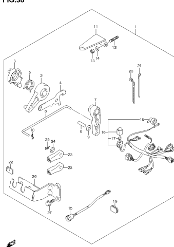
DF15A 2/A P01 013_038 OPT REMOTE CONTROL PARTS
