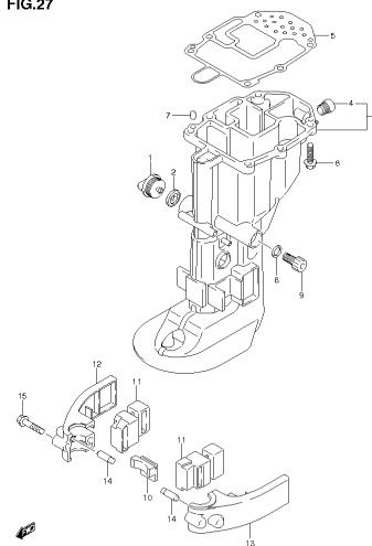
DF15A 20A P01 013_G67 DRIVE SHAFT HOUSING
