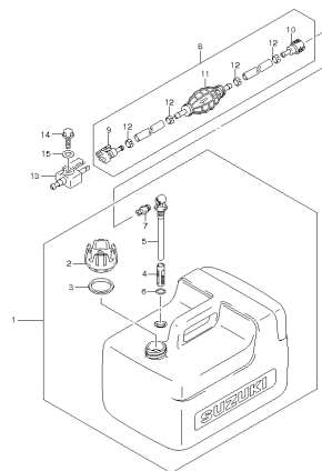
DF15A 2/A P01 013_033 FUEL TANK
