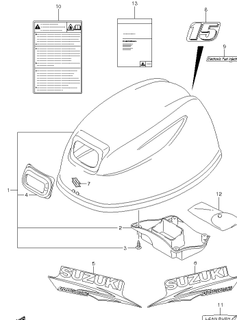
DF15A 20A P01 013_G80 ENGINE COVER
