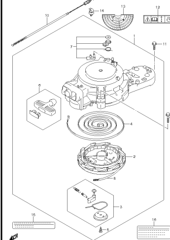
DF15A20A P01 013_012 RECOIL STARTER
