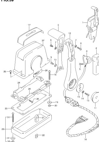
DF15A 2/A P01 013_039 OPT REMOTE CONTROL ASSY SINGLE (1)
