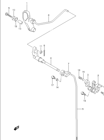
DF15A20A P01 013_015 CLUTCH ROD
