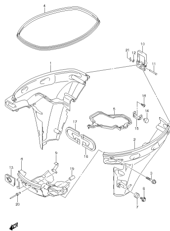
DF15A 20A P01 013_G69 SIDE COVER
