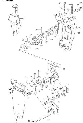
DF15A 2/A P01 013_040 OPT REMOTE CONTROL ASSY SINGLE (2)
