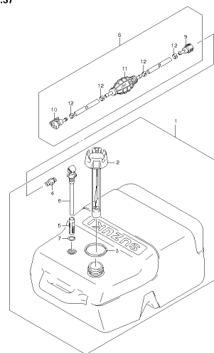
DF15A 2/A P01 013_037 OPT FUEL TANK (RESIN 25L)
