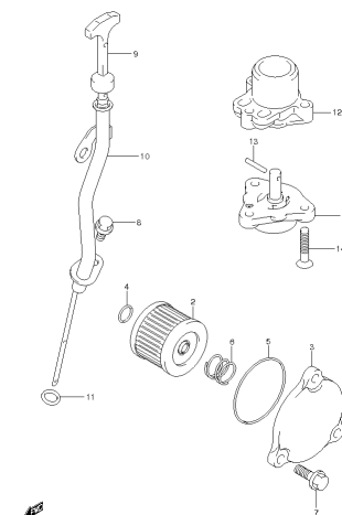
DF15A20A P01 013_014 OIL PUMP
