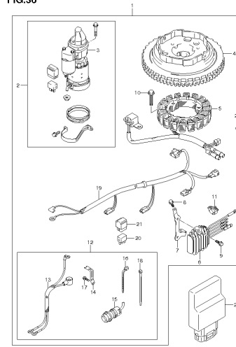
DF15A 2/A P01 013_036 OPT STARTING MOTOR (MANUAL STARTER)
