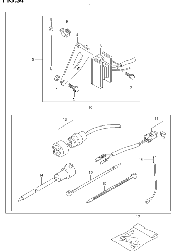
DF15A 2/A P01 013_034 OPT ELECTRICAL (MANUAL STARTER)
