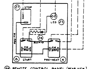
REMOTE CONTROL PANEL (REAR VIEW)
