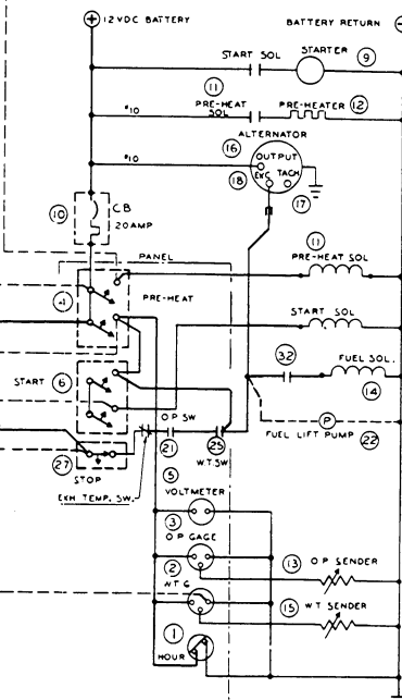
SCHEMATIC DIAGRAM
