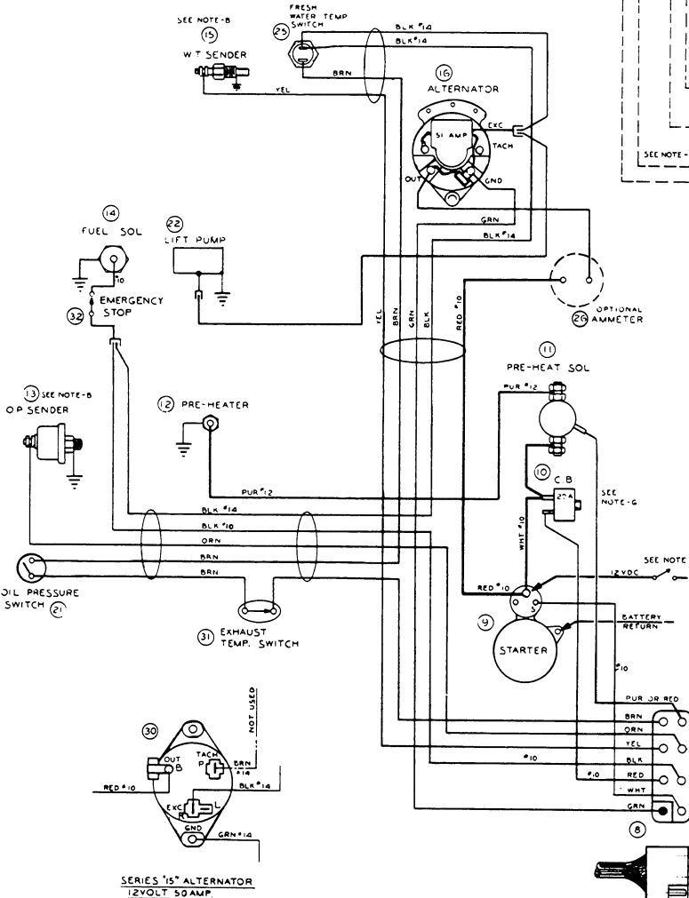
WIRING DIAGRAM
