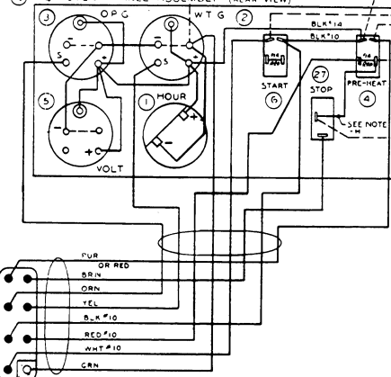
INSTRUMENT PANEL ASSEMBLY (REAR VIEW)
