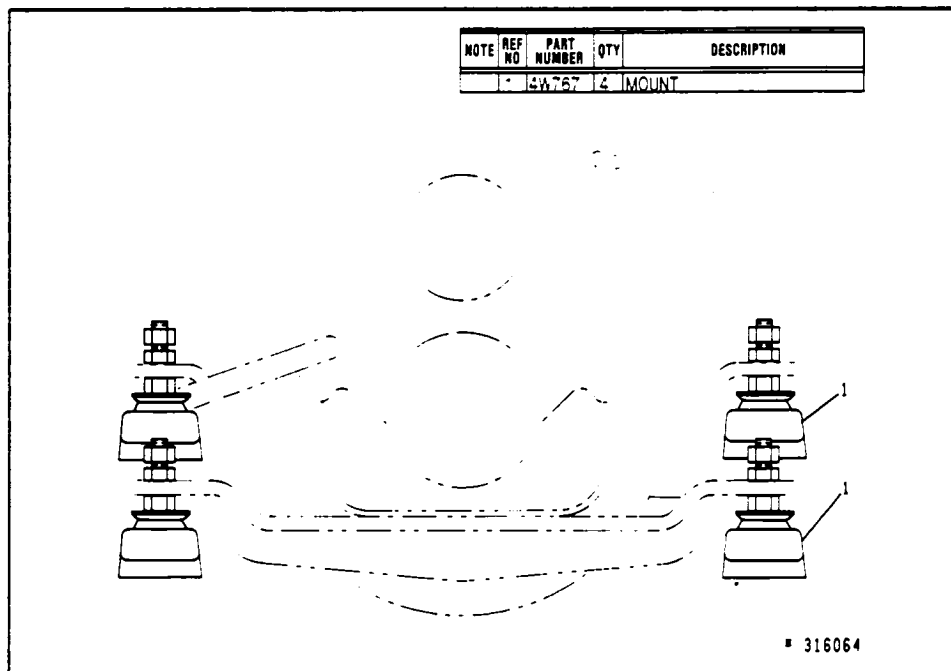
4W1310 ENGINE MOUNTING GROUP-FLEXIBLE Serial No. 123096-Up For Use With 1W9350 Engine Arrangement An Attachment
