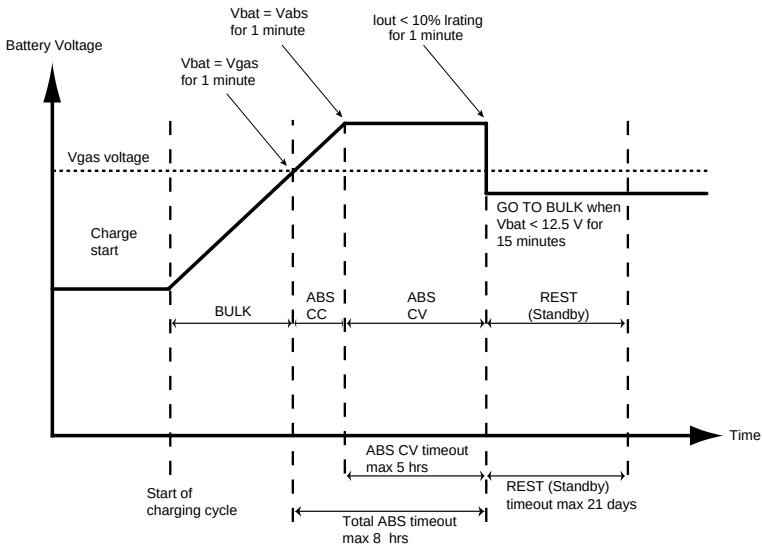
Figure 2-3 Two-Stage Charging Process
