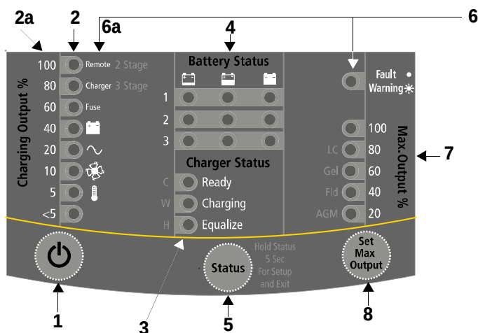
Figure 1-6 Truecharge™ 2 Battery Charger Remote Panel (optional)
