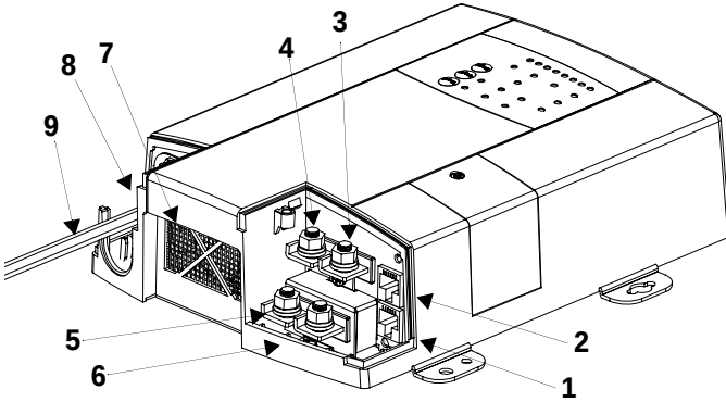
Figure 1-2 Truecharge™ 2 Battery Charger Rear Panel
