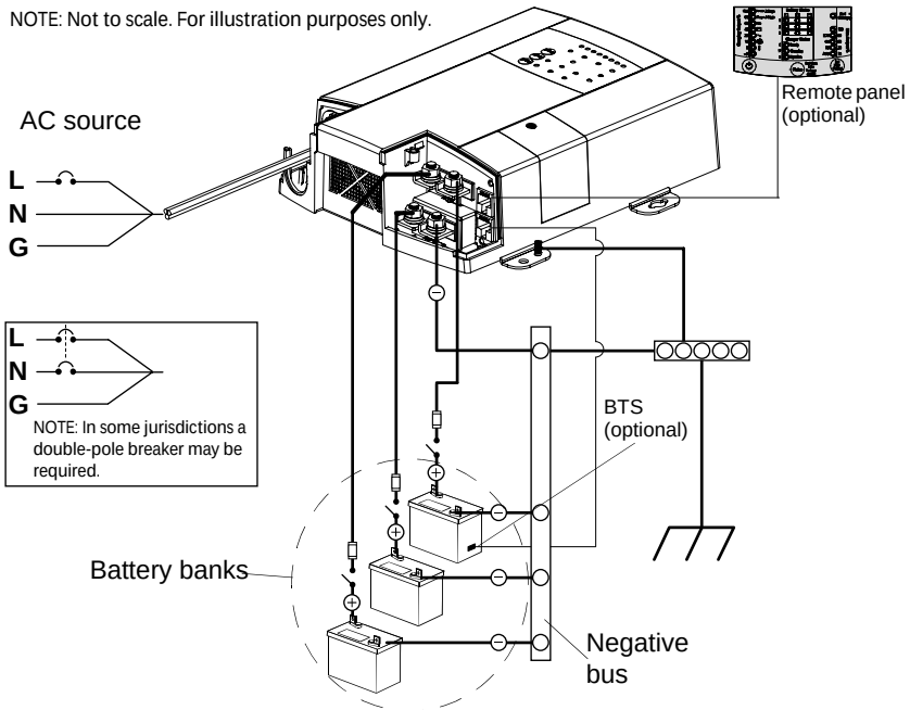
Figure 2-1 Typical Three-Battery Installation
