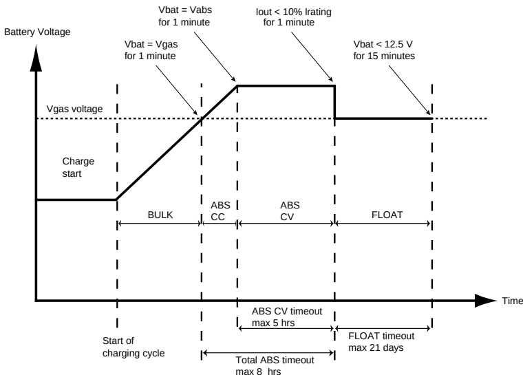
Figure 2-2 Three-Stage Charging Process
