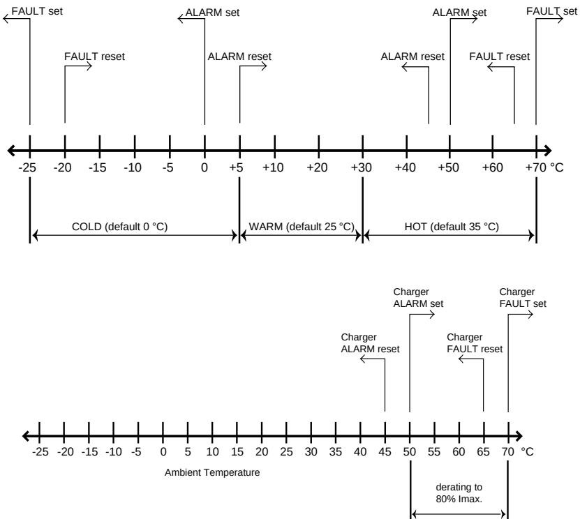
Figure 1-5 Battery and Charger Temperature Thresholds
