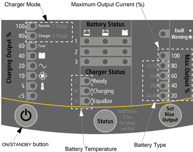
Figure 2-5 Remote Panel
